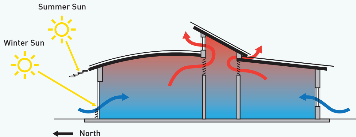
Figure 5: Passive design strategy for community building
