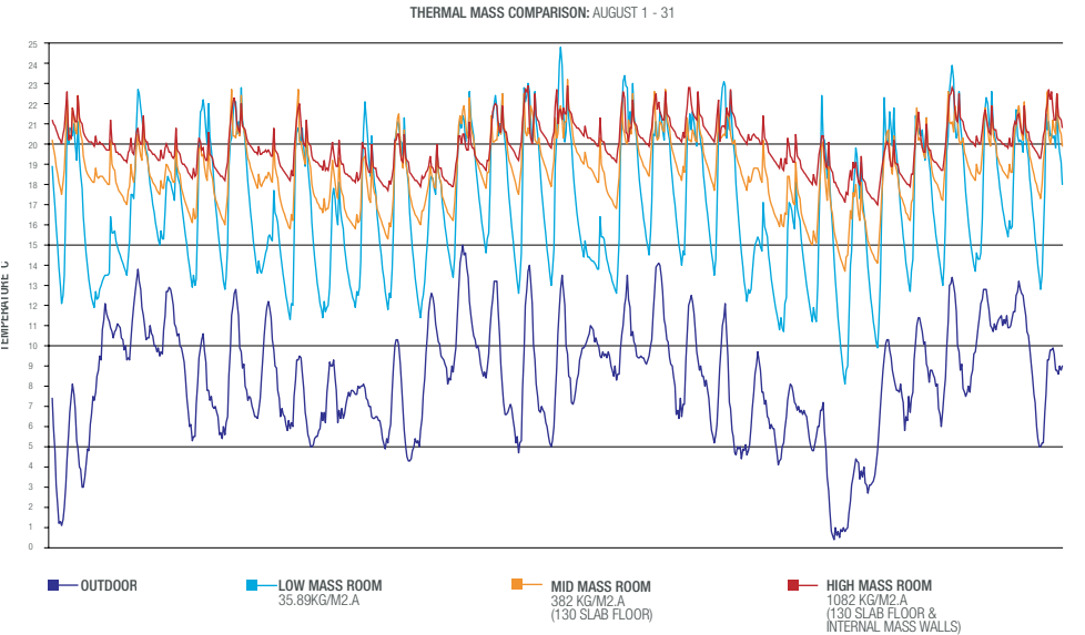
Fig. 6 Expected temperature profiles for the low-mass, mid-mass and high-mass building type for August. (AccuRate, climate zone 26, Hobart)
