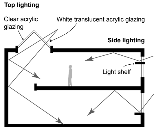
Figure 4. Top versus side lighting (Energy Design Resources 1999).
