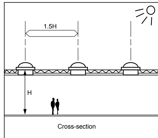
Figure 5. Rule of thumb for spacing skylights to help achieve uniform illuminance (HMG 1998).
