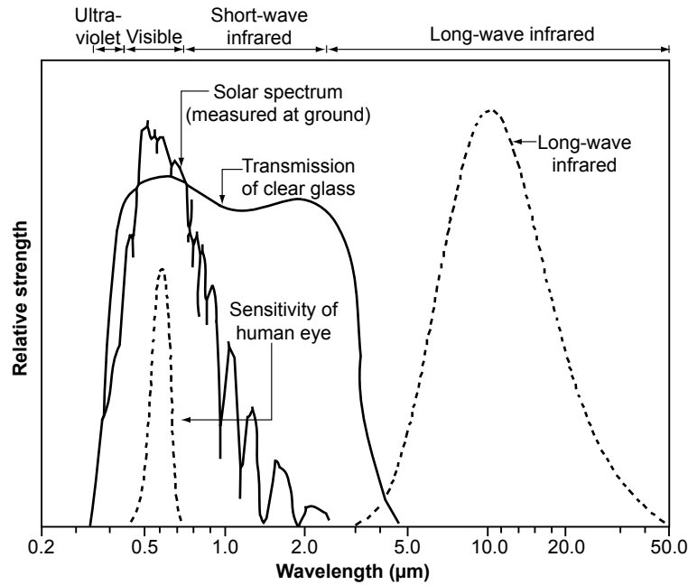
Figure 1. The solar spectrum and transmittance of clear glass.
