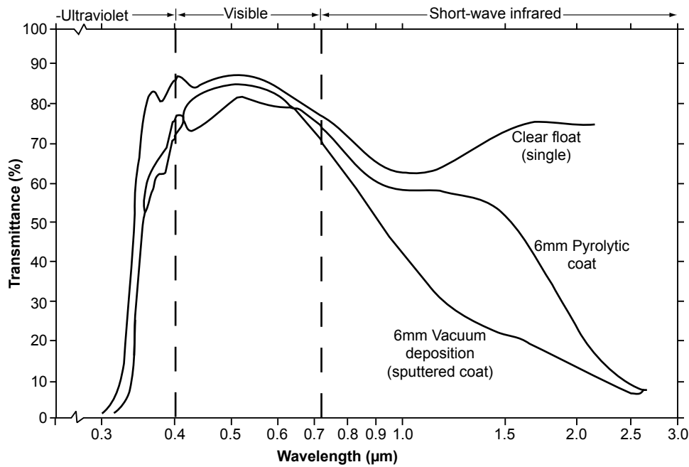
Figure 2. Spectral behaviour of pyrolytic and sputtered low-e coatings.
